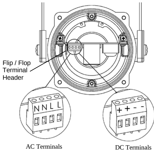
Fig. 4 Internal View of BExBGD 5 Joule Beacon
