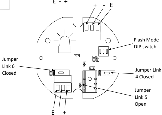
D105HDC024 Beacon PCBA (12VDC Mode – Customer to Set)
